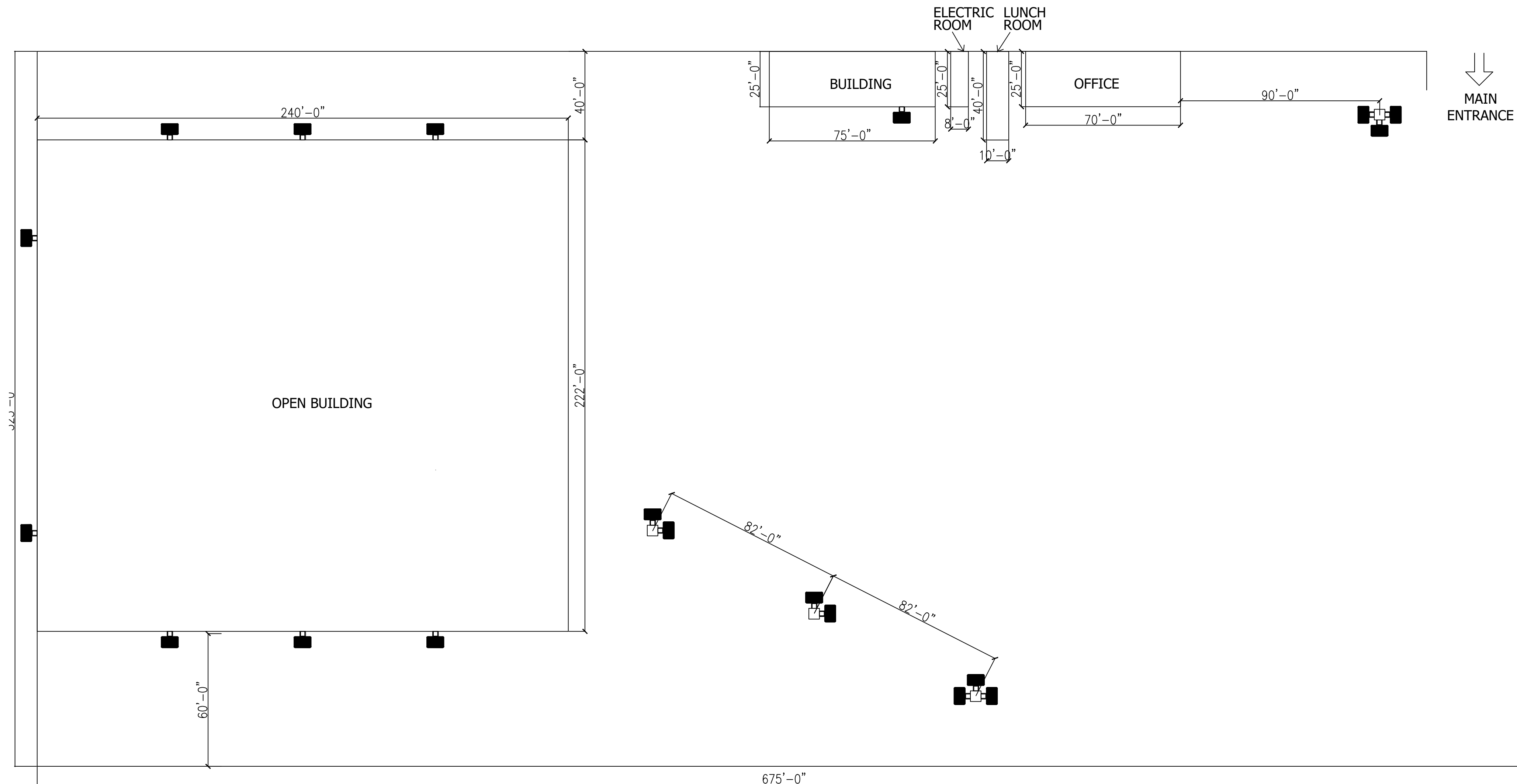
SUBJECT PROPERTY (OUTDOOR LIGHTING PLAN) SCALE: 1/32"=1'-0"
