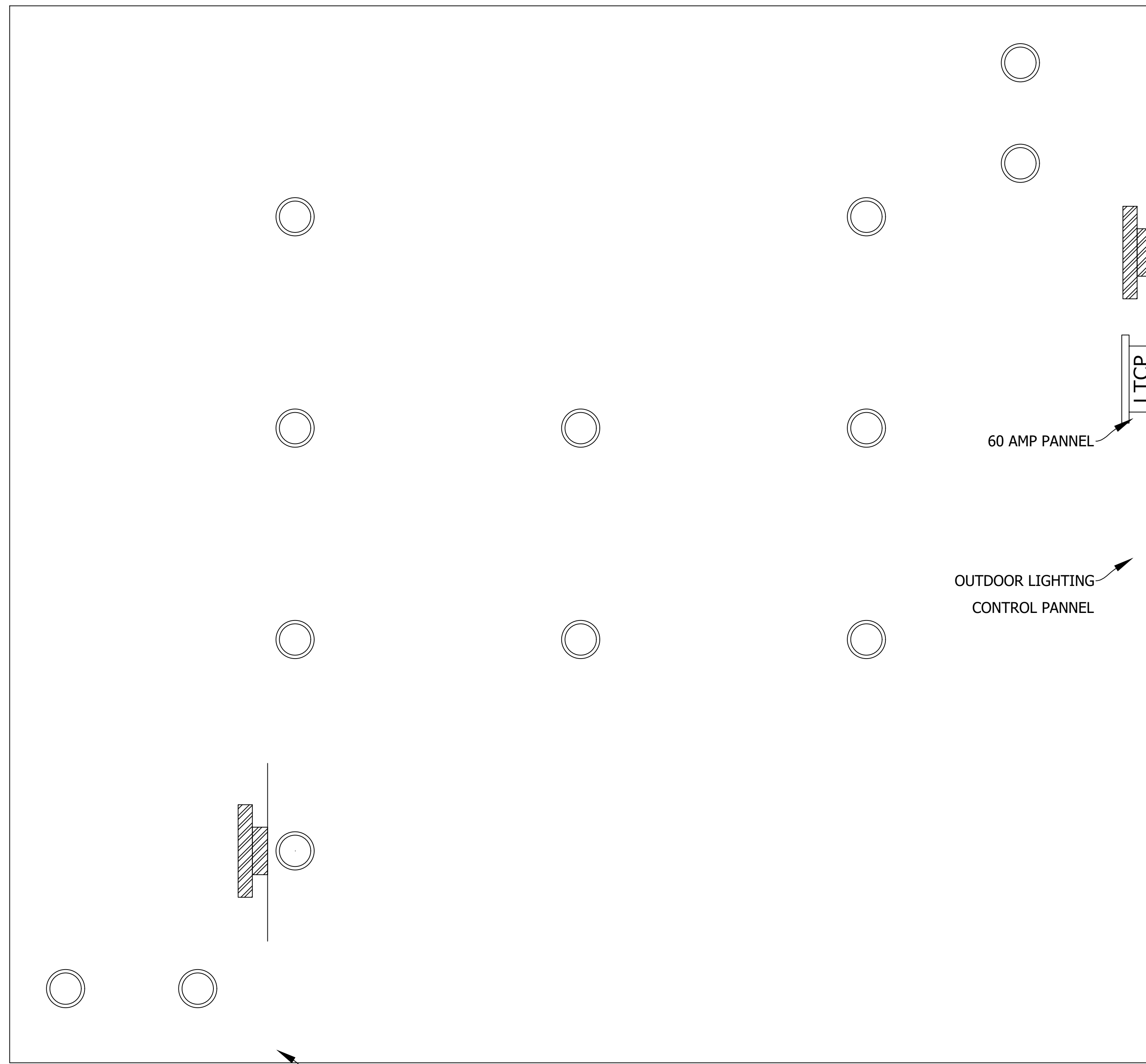
OPEN BUILDING INDOOR LIGHTING PLAN (222' X 252') SCALE: 1/16"=1'-0"
