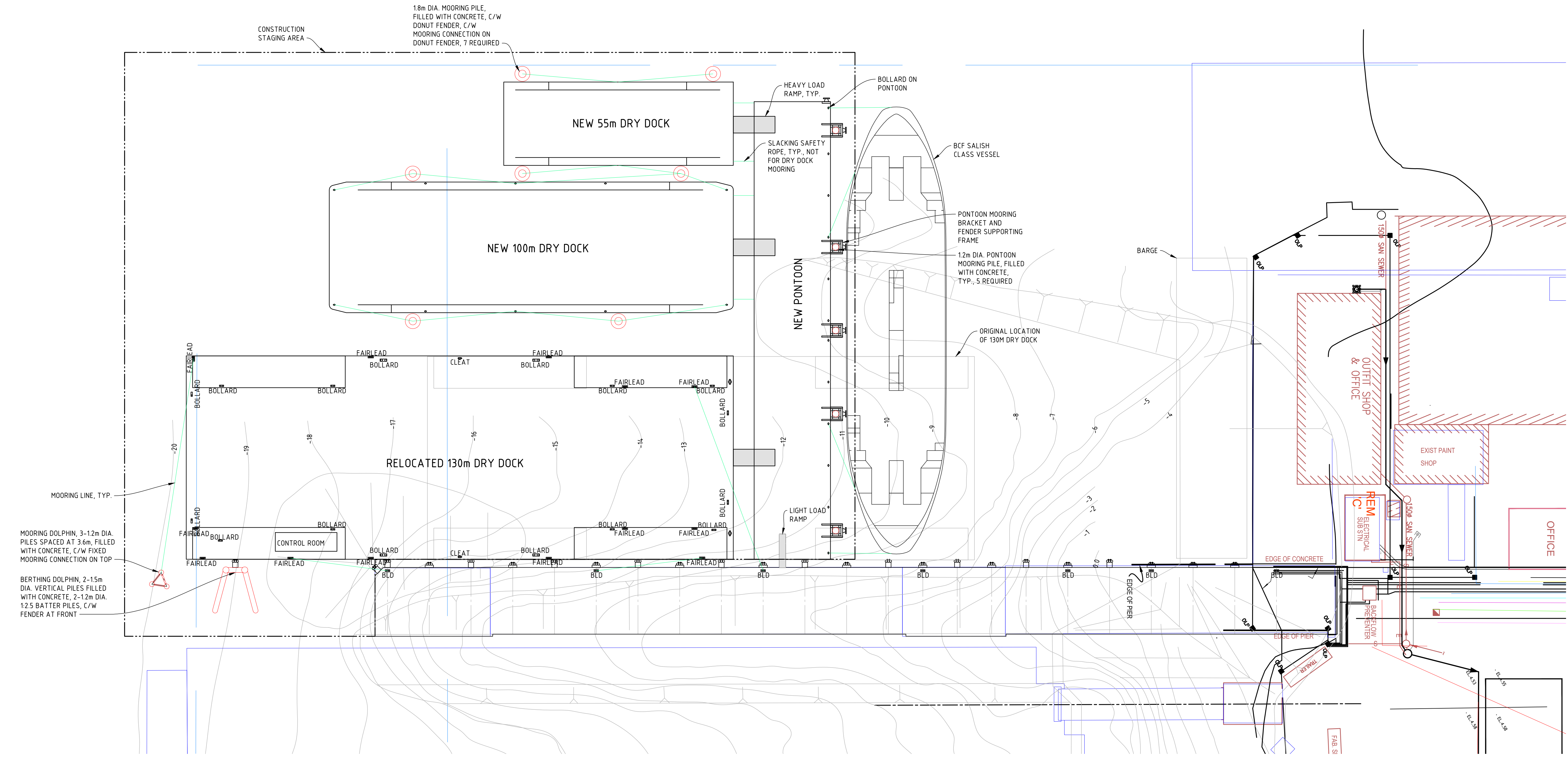
PLAN 1:500
